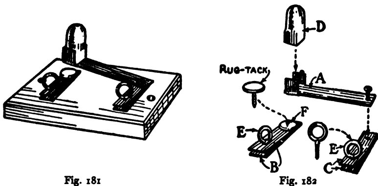
FIG. 181. — A Home-Made Switch.
